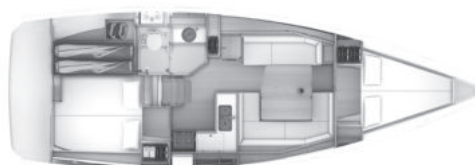
Version A 1 cabina a prua, 1 cabina a poppa, 1 bagno
